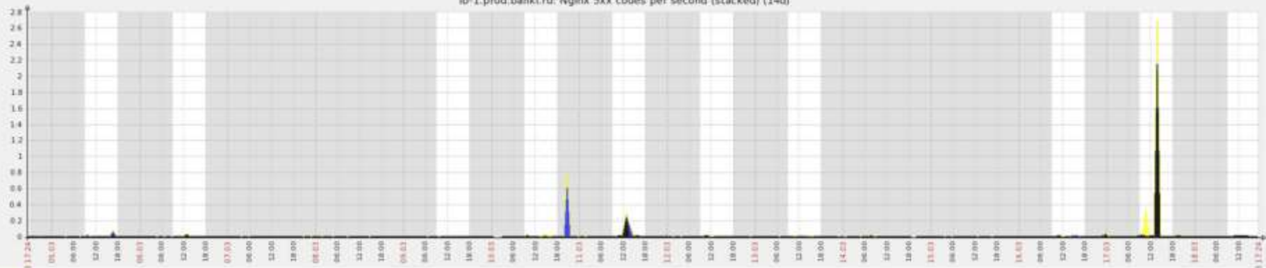
fb-1.prod.banki.ru: Nginx 5xx codes per second (stacked) (14d)
